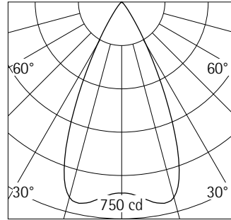
LED 6W 600lm 3000K warm white
